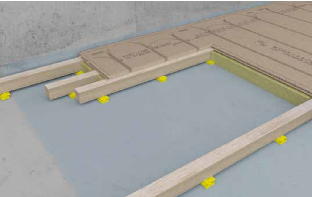
Joist positioning CC from the wall: first 3.5 cm, second 17.5 cm, and third 31.2 cm.
